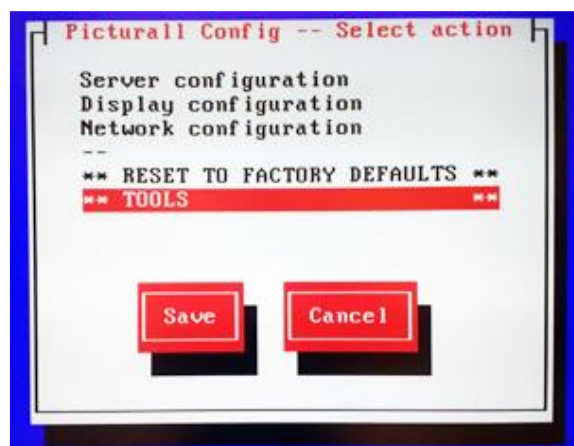
Fig. 49 - Configuration mode
