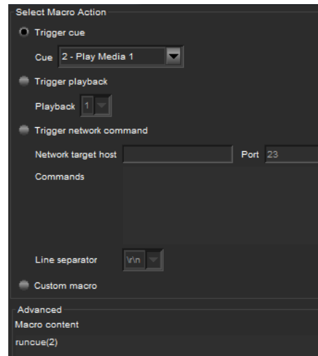
Fig. 114 - Cue macro
