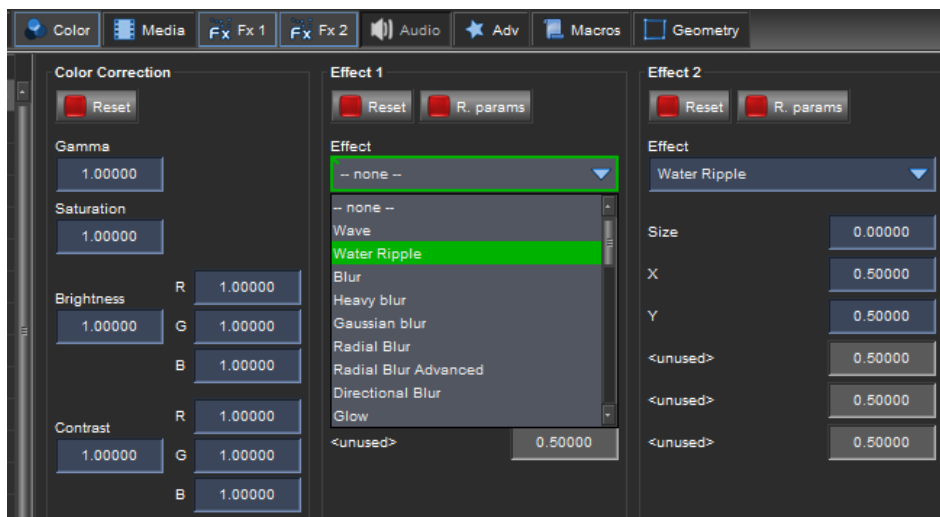
Fig. 91 - Effects
