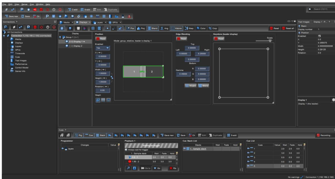
Fig. 50 - Picturall Commander
