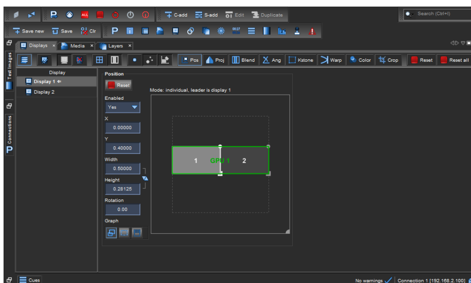
Fig. 62 - Positioning panel
