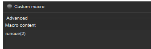
Fig. 115 - Macro content
